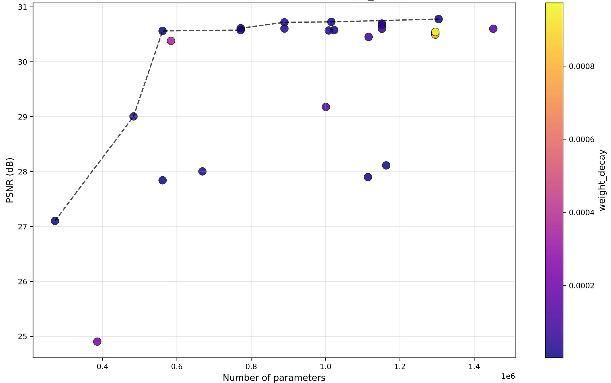
PSNR vs #Params — OmniSR — by weight_decay
